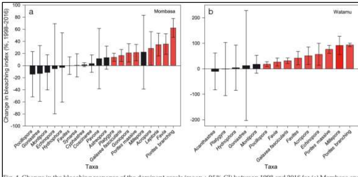
Figure 39: Changes in bleaching response in Mombasa and Watamu MCA. (Source: McClanahan 2017)
